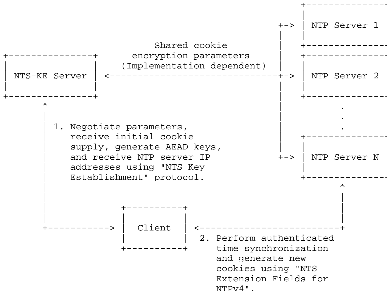
Figure 1: Overview of High-Level Interactions in NTS
