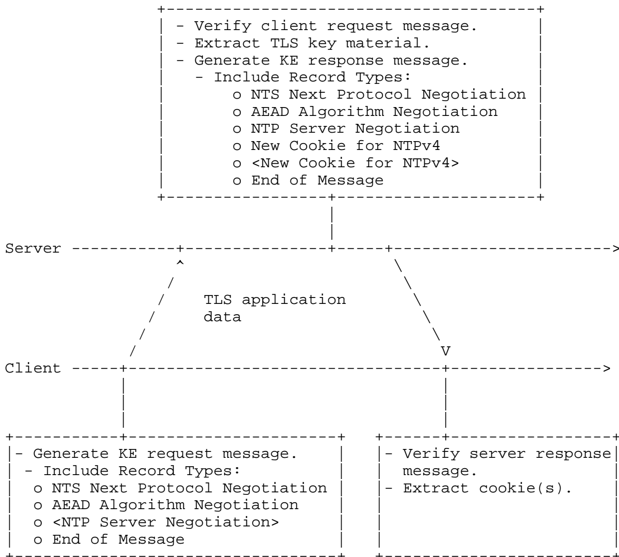
Figure 3: NTS Key Exchange Messages
