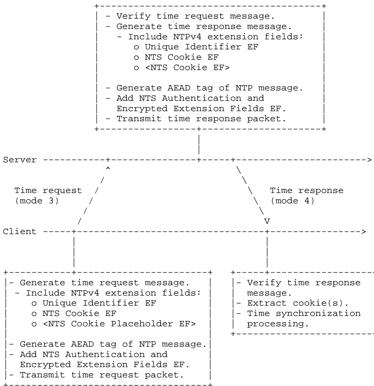
Figure 5: NTS Time Synchronization Messages
